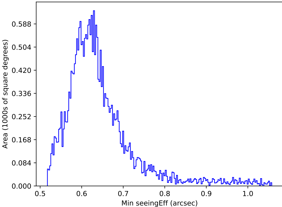
too_ignore_100_1v3.4_10yrs All sky r band: Min seeingEff
