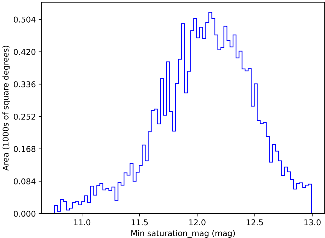
too_ignore_100_1v3.4_10yrs WFD z band: Min saturation_mag
