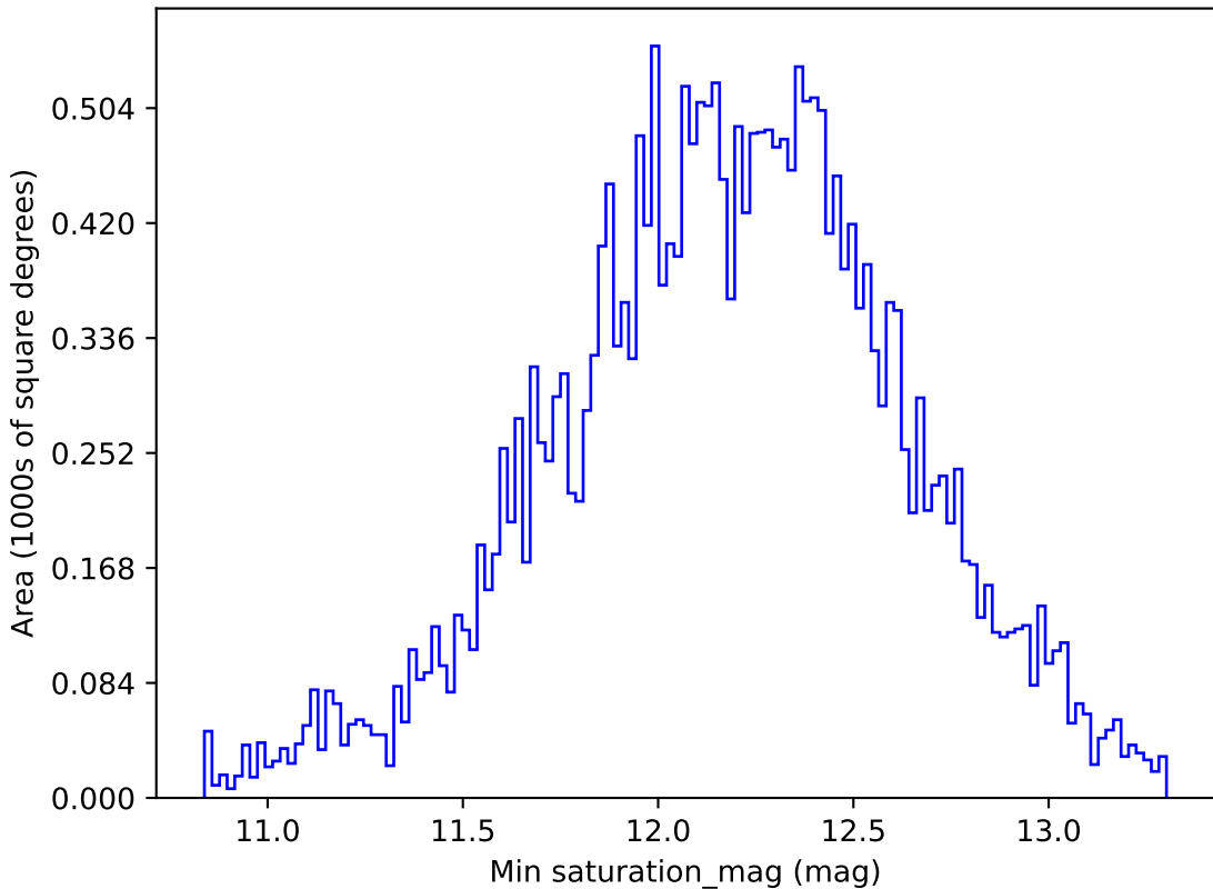
too_ignore_100_1v3.4_10yrs All sky z band: Min saturation_mag
