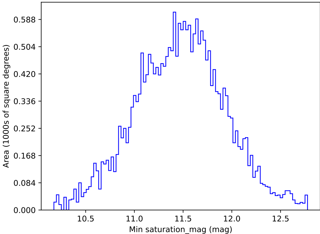
too_ignore_100_1v3.4_10yrs All sky u band: Min saturation_mag
