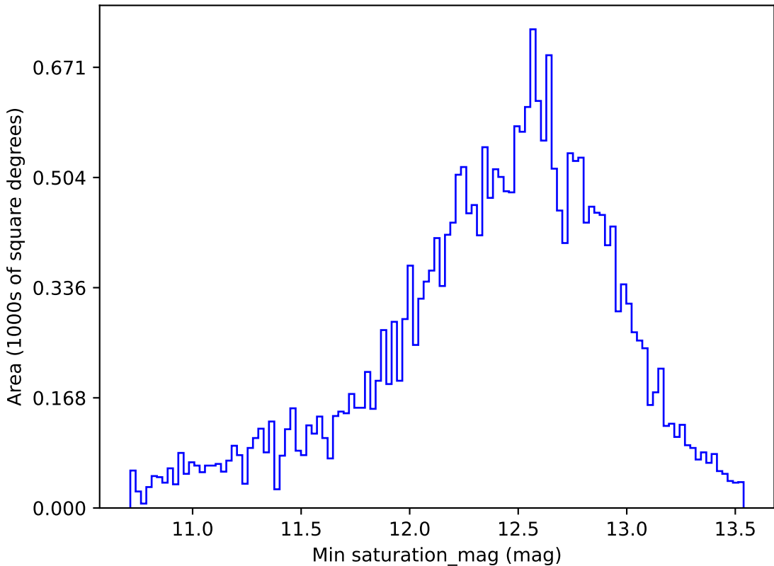
too_ignore_100_1v3.4_10yrs All sky i band: Min saturation_mag
