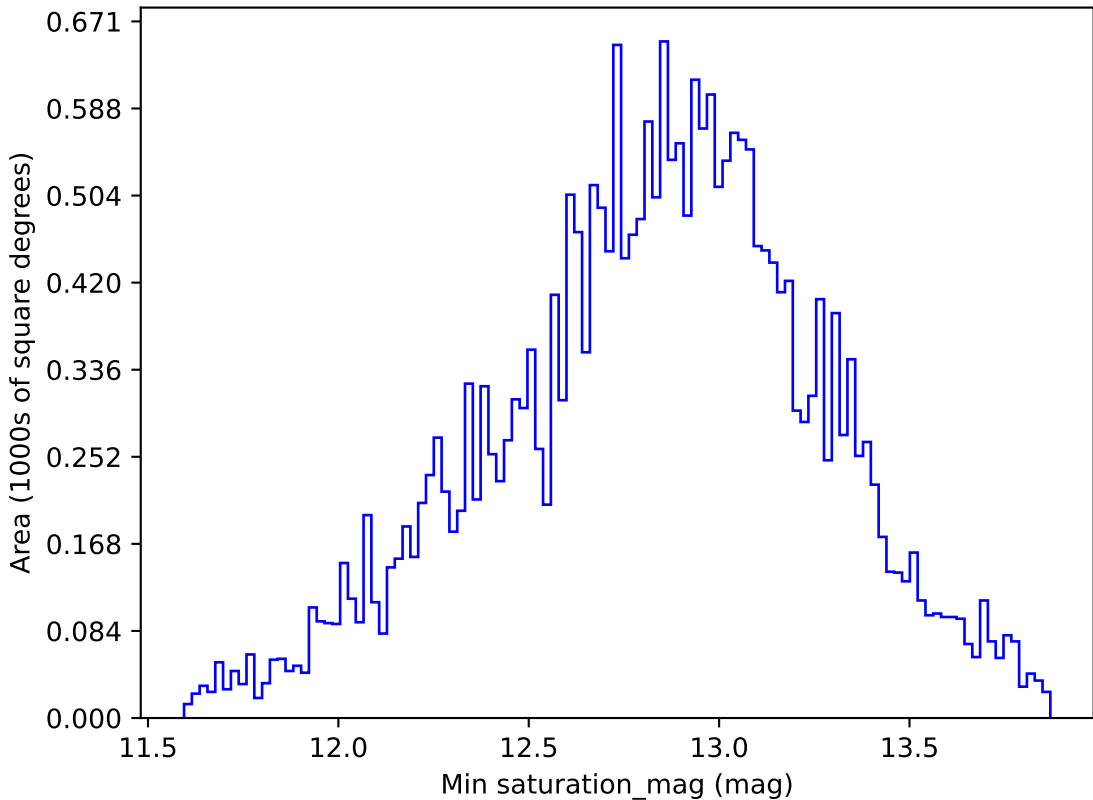
too_ignore_100_1v3.4_10yrs All sky g band: Min saturation_mag
