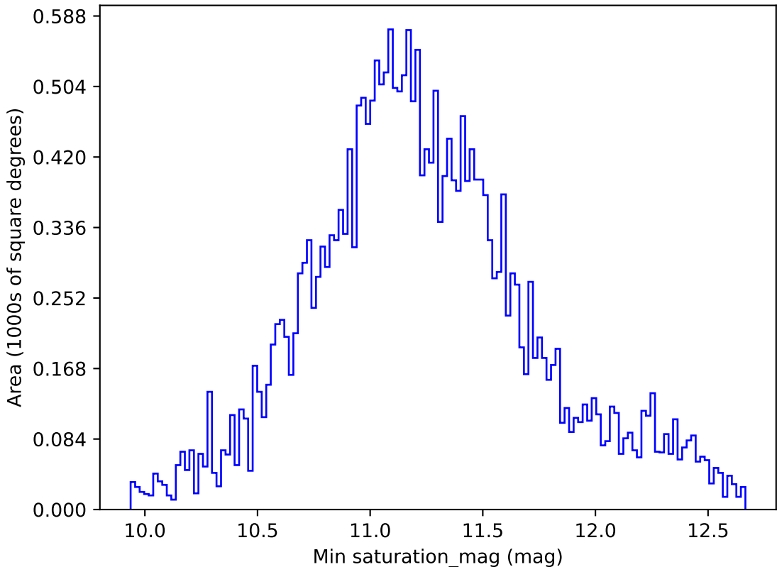
too_ignore_100_1v3.4_10yrs All sky all bands: Min saturation_mag
