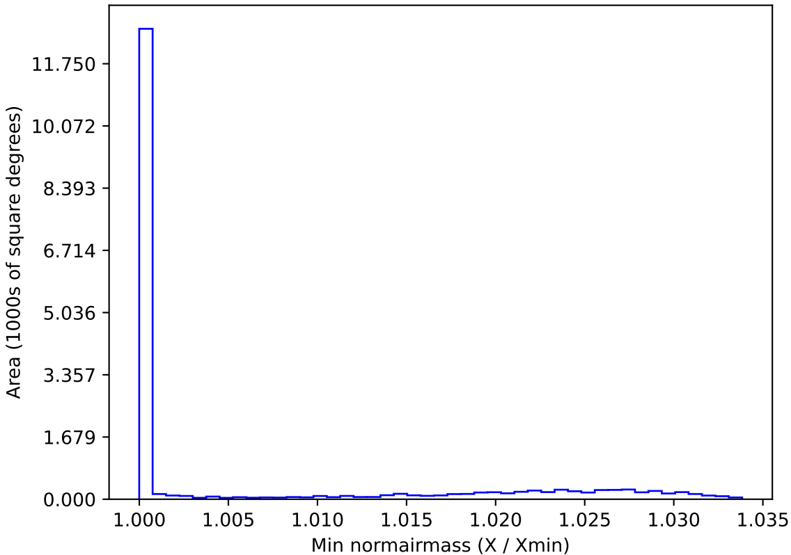
too_ignore_100_1v3.4_10yrs WFD i band: Min normairmass
