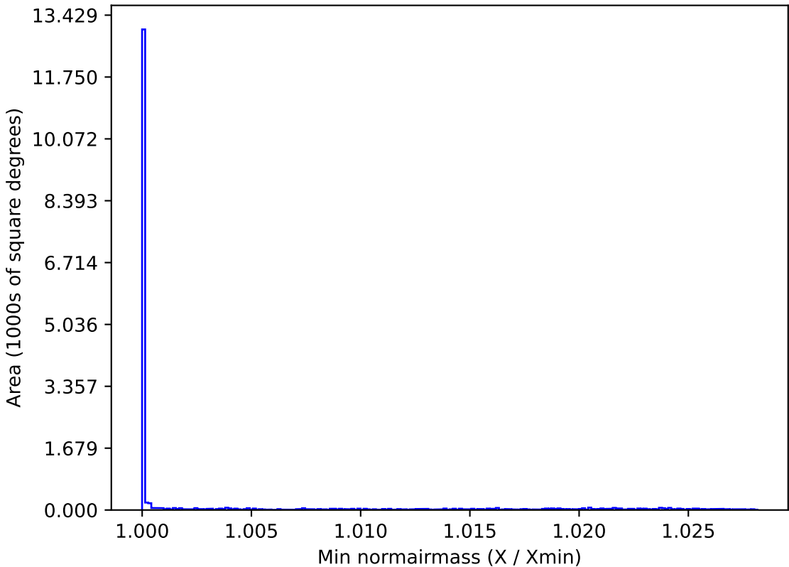
too_ignore_100_1v3.4_10yrs WFD all bands: Min normairmass
