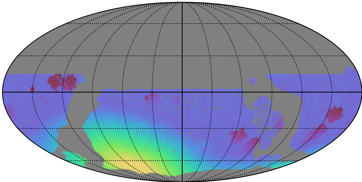
too_ignore_100_1v3.4_10yrs WFD z band: Min moonDistance
