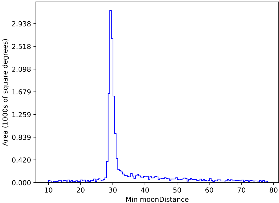
too_ignore_100_1v3.4_10yrs WFD z band: Min moonDistance
