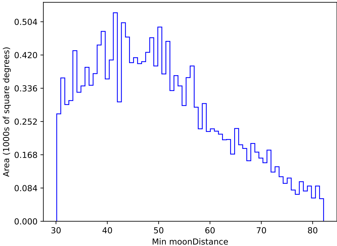
too_ignore_100_1v3.4_10yrs WFD u band: Min moonDistance
