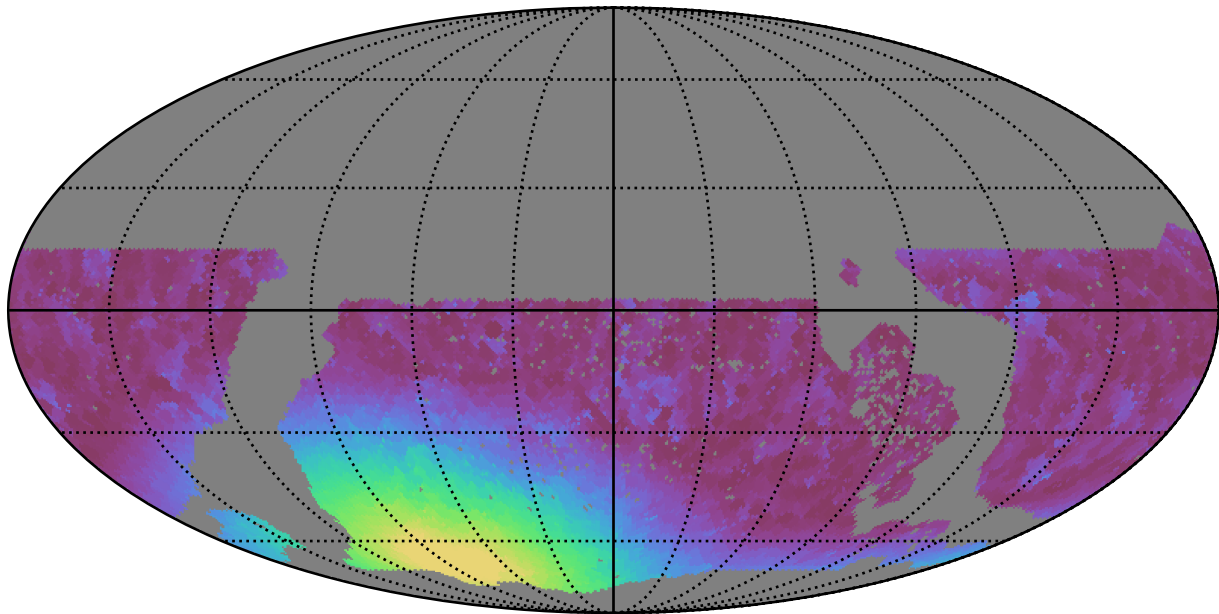
too_ignore_100_1v3.4_10yrs WFD r band: Min moonDistance
