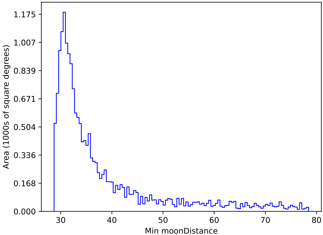
too_ignore_100_1v3.4_10yrs WFD r band: Min moonDistance
