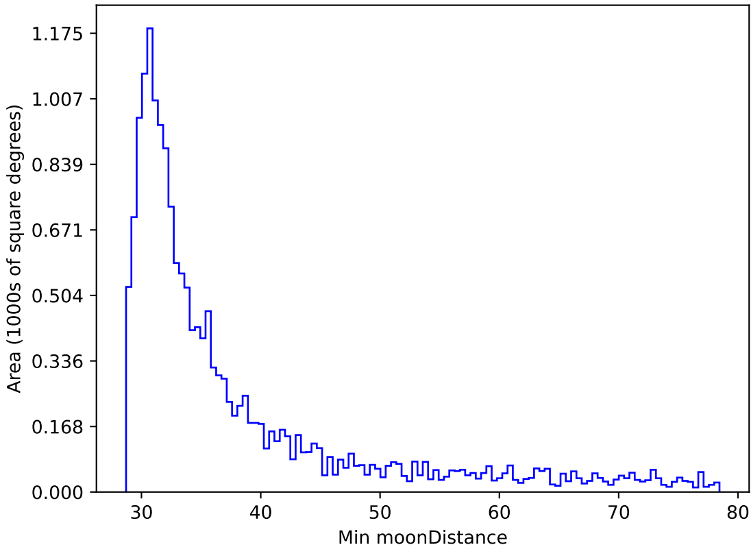
too_ignore_100_1v3.4_10yrs WFD r band: Min moonDistance
