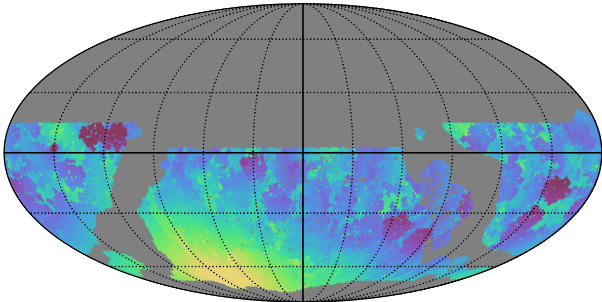
too_ignore_100_1v3.4_10yrs WFD g band: Min moonDistance
