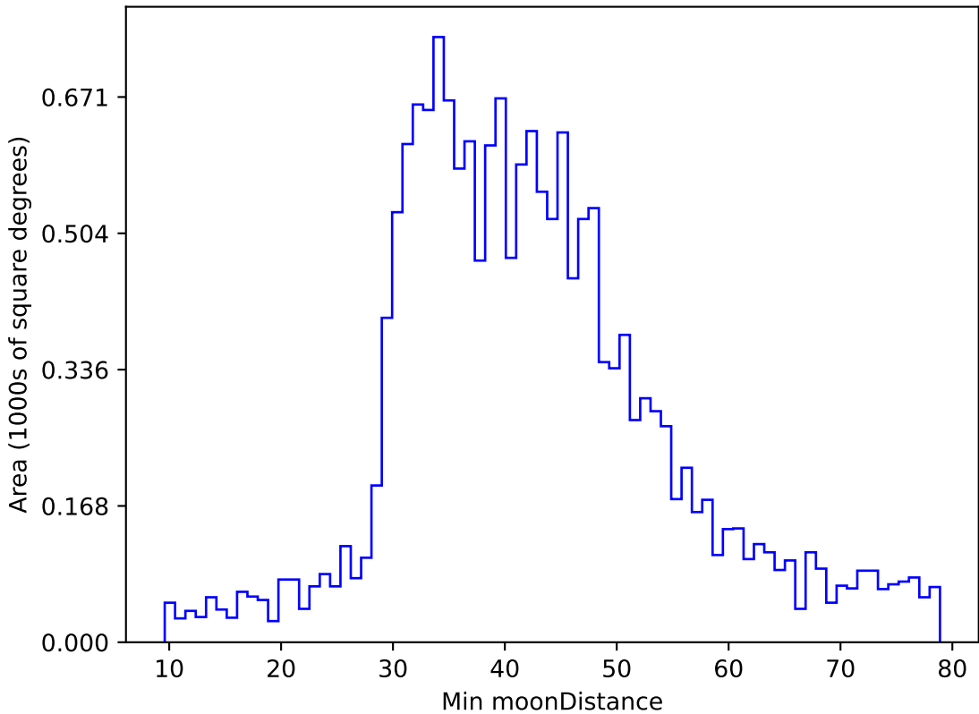
too_ignore_100_1v3.4_10yrs WFD g band: Min moonDistance
