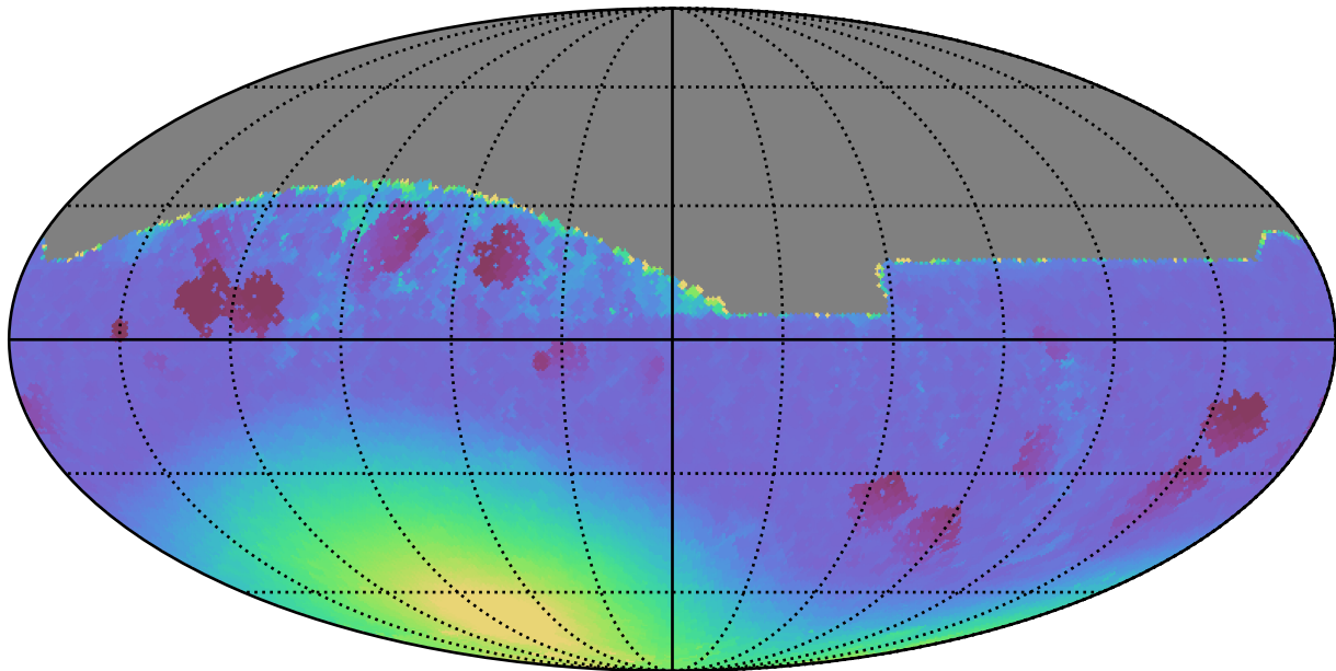
too_ignore_100_1v3.4_10yrs All sky z band: Min moonDistance
