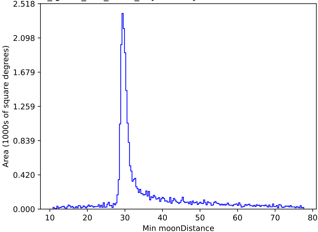
too_ignore_100_1v3.4_10yrs All sky z band: Min moonDistance
