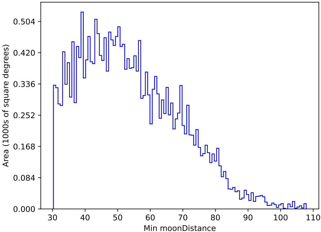
too_ignore_100_1v3.4_10yrs All sky u band: Min moonDistance
