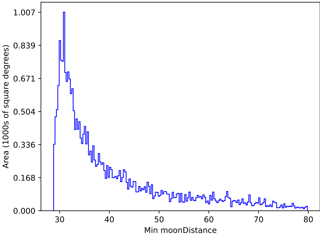
too_ignore_100_1v3.4_10yrs All sky r band: Min moonDistance
