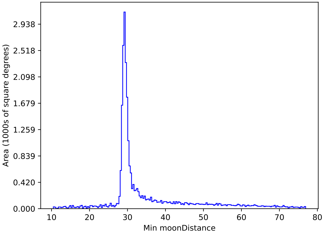
too_ignore_100_1v3.4_10yrs All sky all bands: Min moonDistance
