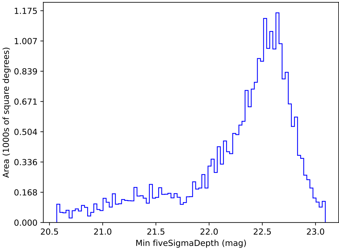
too_ignore_100_1v3.4_10yrs Yr 1 z band: Min fiveSigmaDepth
