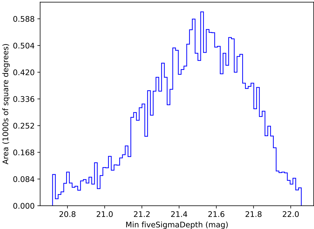
too_ignore_100_1v3.4_10yrs Yr 1 y band: Min fiveSigmaDepth
