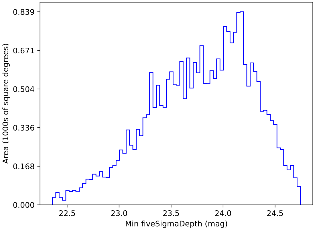
too_ignore_100_1v3.4_10yrs Yr 1 g band: Min fiveSigmaDepth
