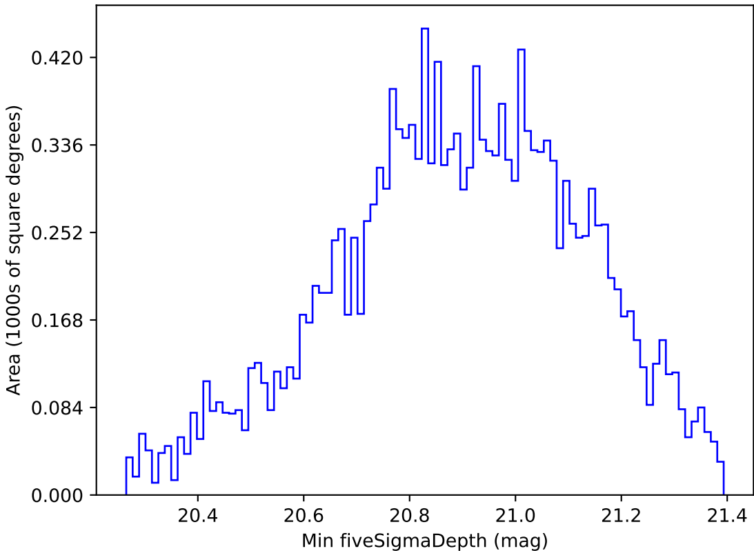
too_ignore_100_1v3.4_10yrs WFD y band: Min fiveSigmaDepth
