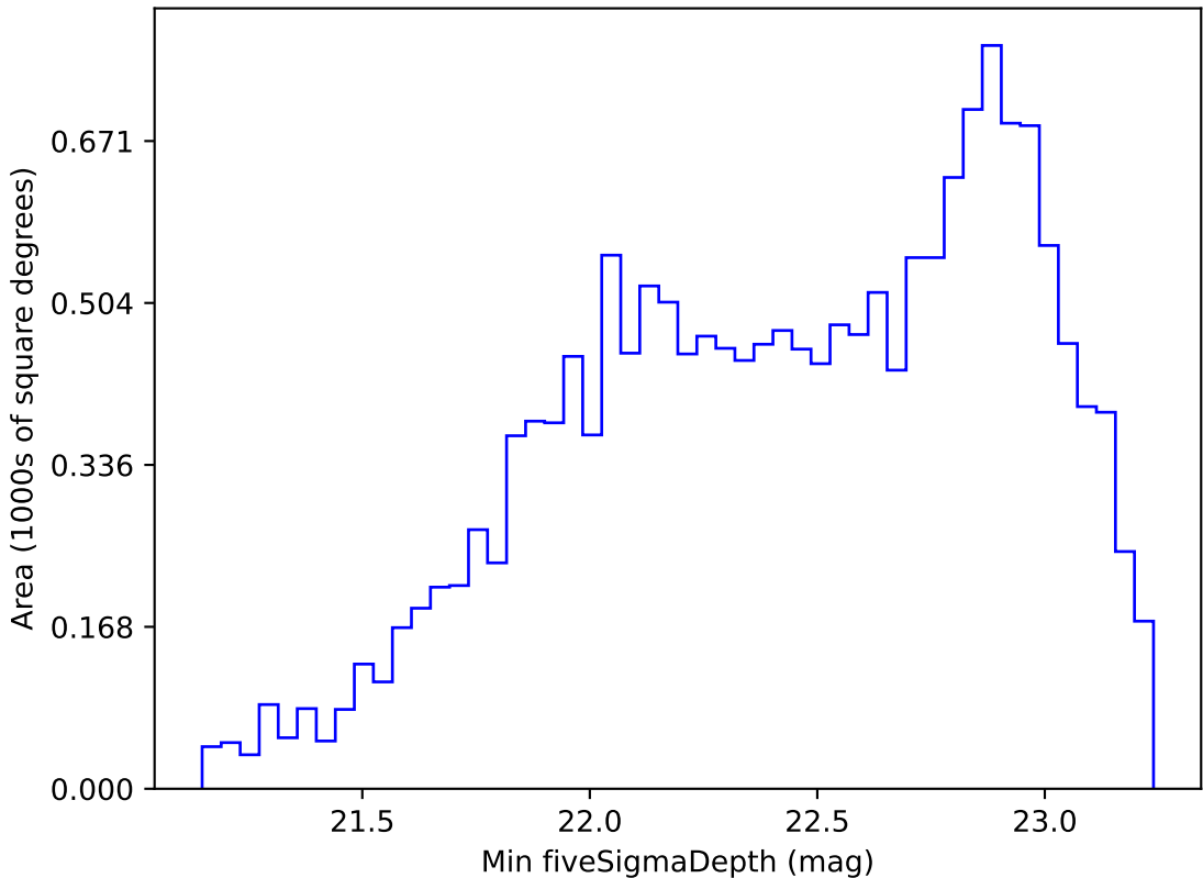
too_ignore_100_1v3.4_10yrs WFD r band: Min fiveSigmaDepth
