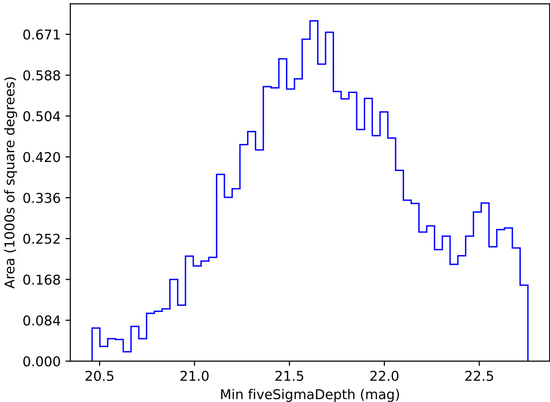
too_ignore_100_1v3.4_10yrs WFD i band: Min fiveSigmaDepth
