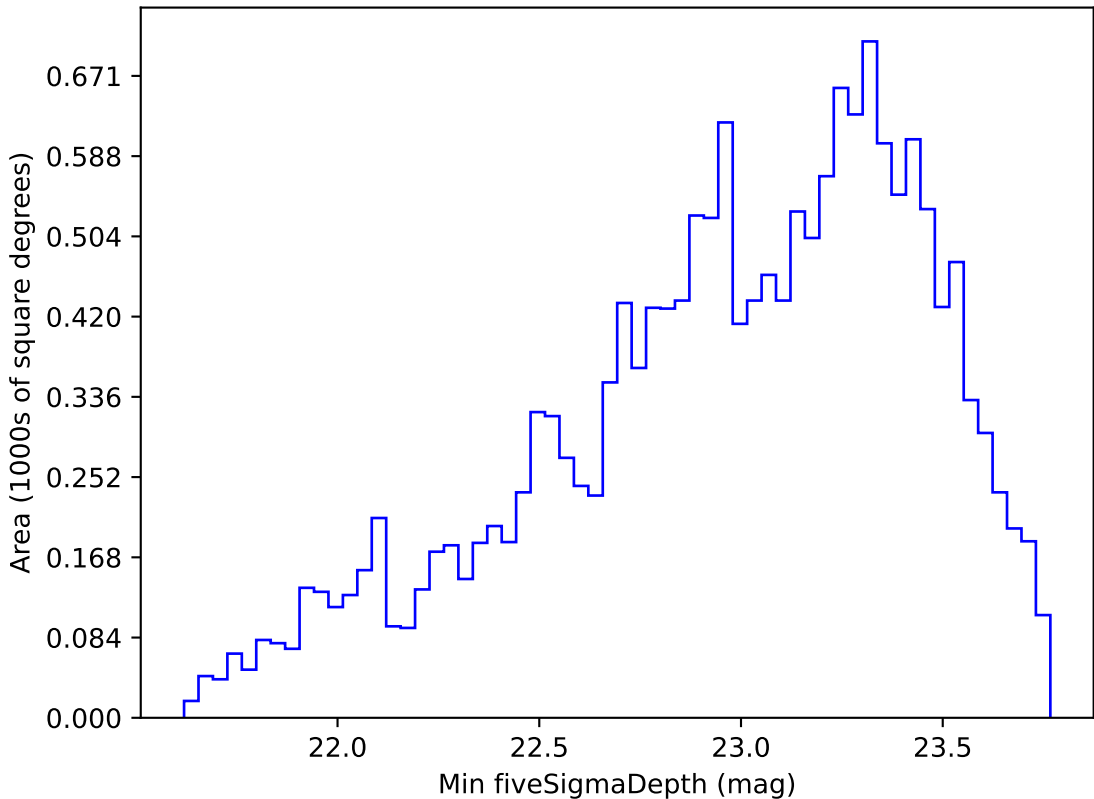
too_ignore_100_1v3.4_10yrs WFD g band: Min fiveSigmaDepth
