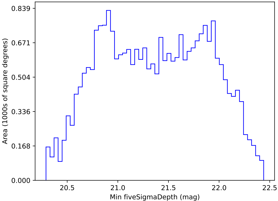
too_ignore_100_1v3.4_10yrs All sky z band: Min fiveSigmaDepth
