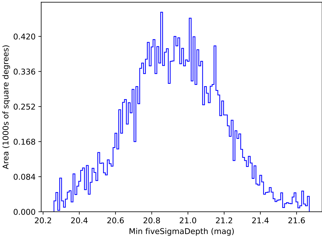
too_ignore_100_1v3.4_10yrs All sky y band: Min fiveSigmaDepth
