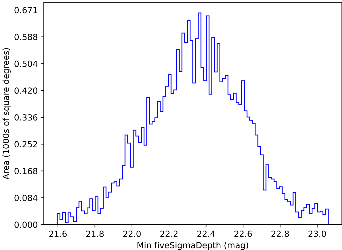
too_ignore_100_1v3.4_10yrs All sky u band: Min fiveSigmaDepth
