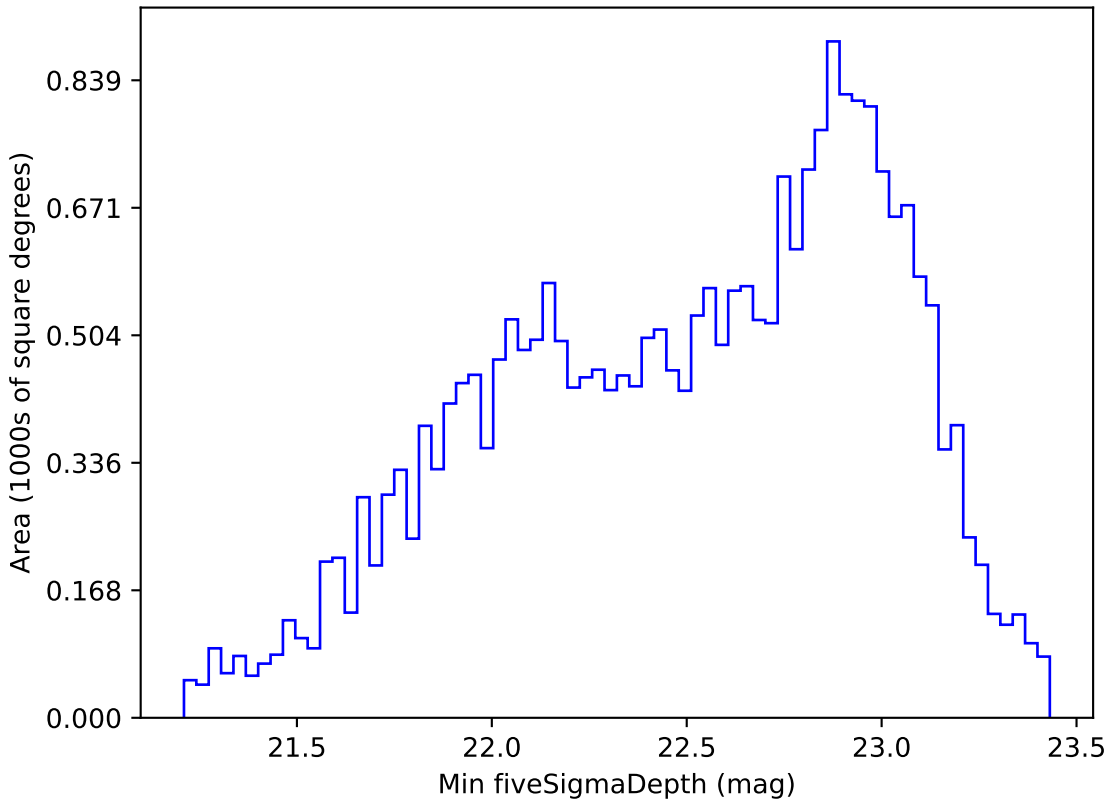
too_ignore_100_1v3.4_10yrs All sky r band: Min fiveSigmaDepth
