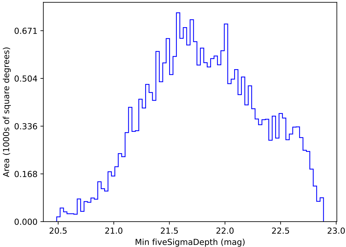
too_ignore_100_1v3.4_10yrs All sky i band: Min fiveSigmaDepth
