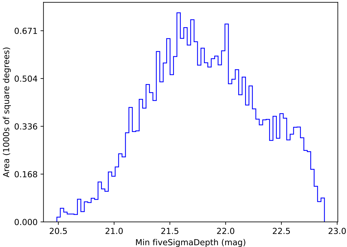
too_ignore_100_1v3.4_10yrs All sky i band: Min fiveSigmaDepth
