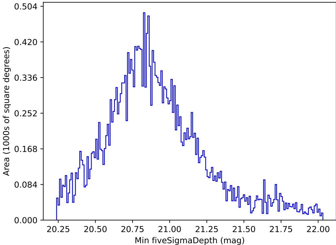
too_ignore_100_1v3.4_10yrs All sky all bands: Min fiveSigmaDepth
