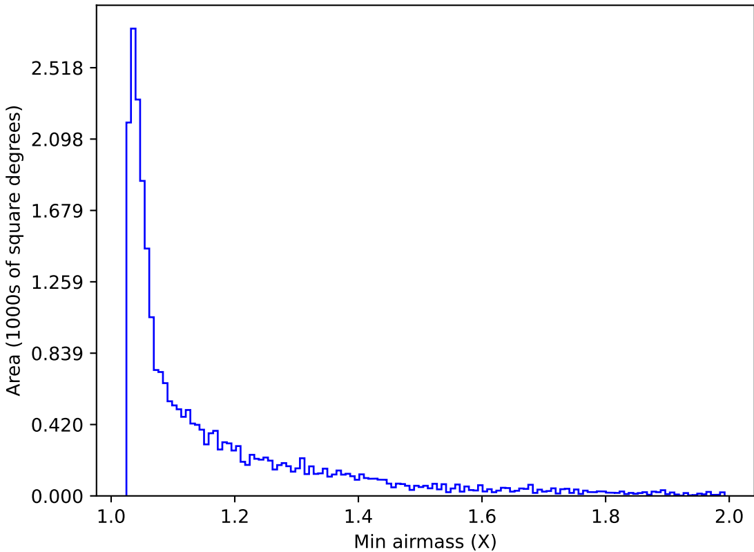
too_ignore_100_1v3.4_10yrs Yr 1 z band: Min airmass
