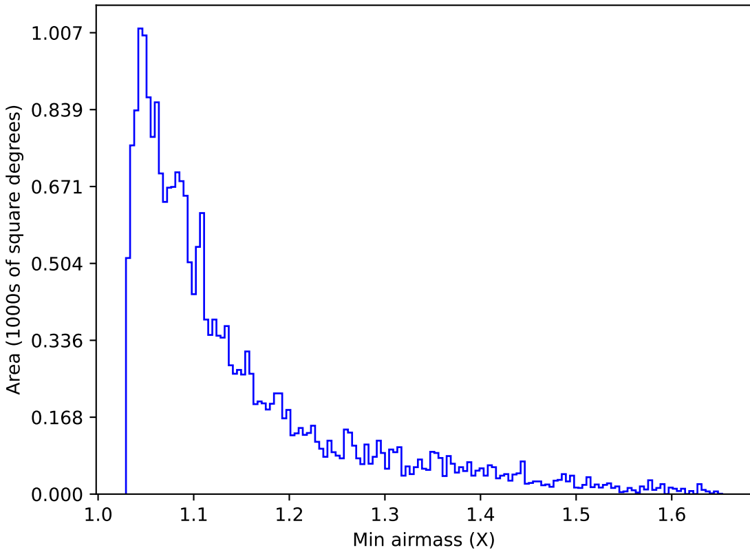
too_ignore_100_1v3.4_10yrs Yr 1 u band: Min airmass
