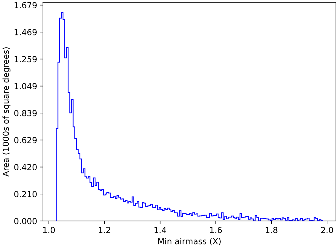
too_ignore_100_1v3.4_10yrs Yr 1 g band: Min airmass
