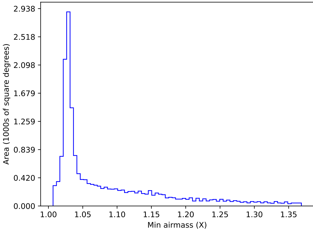
too_ignore_100_1v3.4_10yrs WFD z band: Min airmass
