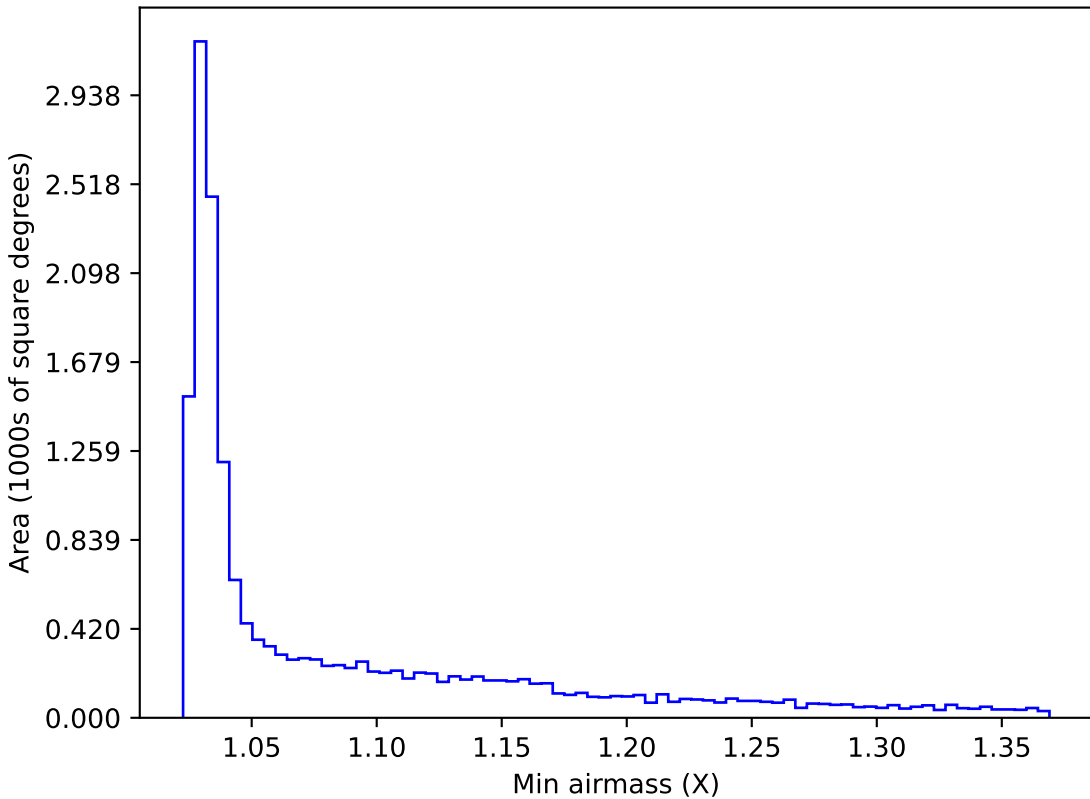
too_ignore_100_1v3.4_10yrs WFD y band: Min airmass
