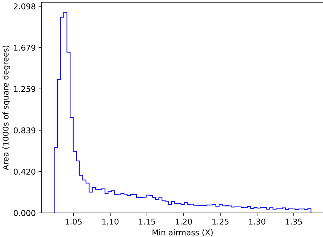
too_ignore_100_1v3.4_10yrs WFD u band: Min airmass
