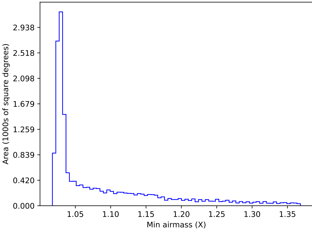
too_ignore_100_1v3.4_10yrs WFD i band: Min airmass
