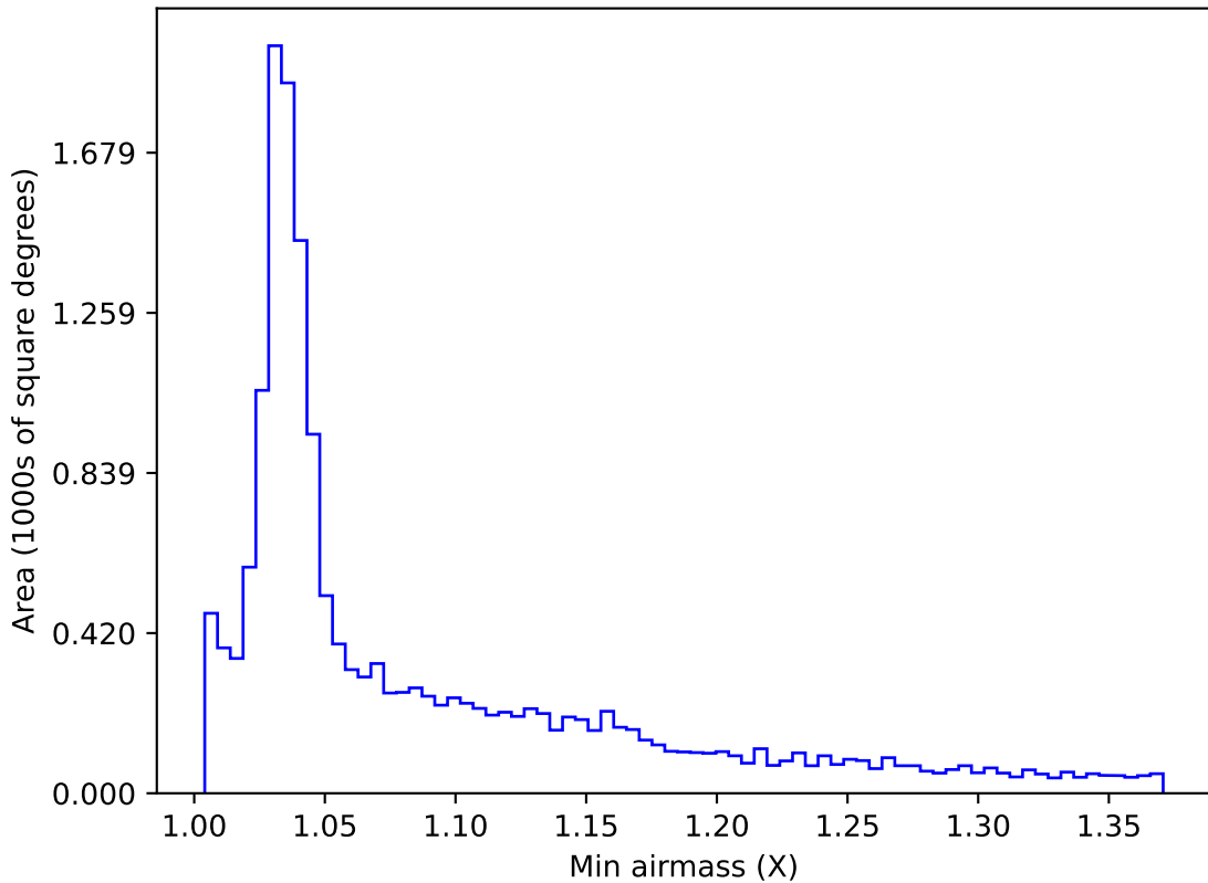
too_ignore_100_1v3.4_10yrs WFD g band: Min airmass
