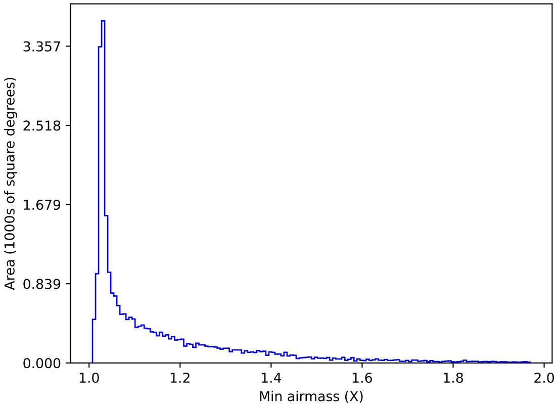
too_ignore_100_1v3.4_10yrs All sky z band: Min airmass
