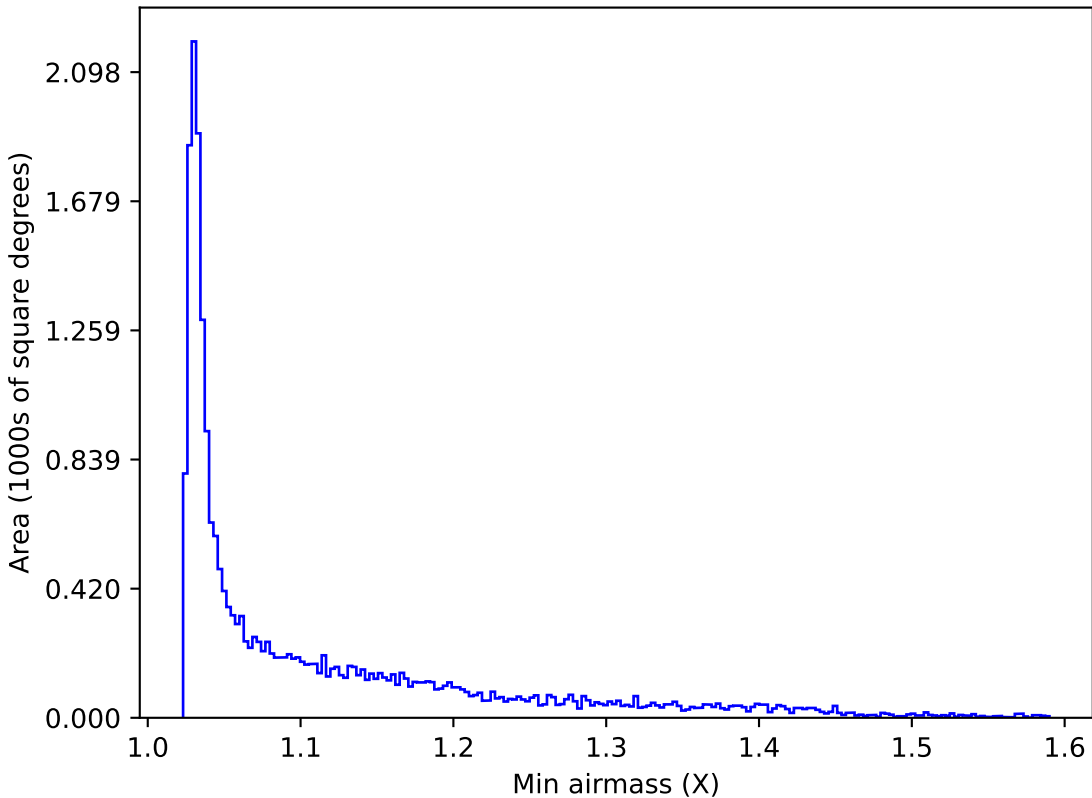
too_ignore_100_1v3.4_10yrs All sky y band: Min airmass
