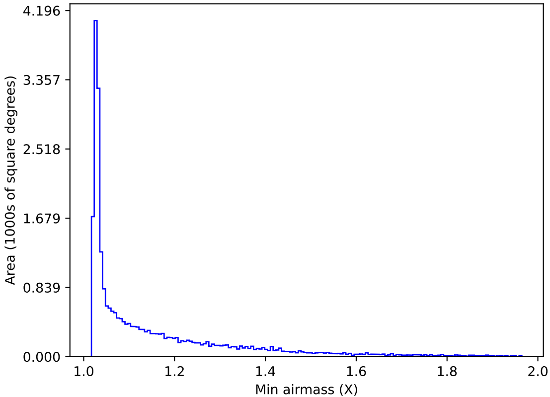
too_ignore_100_1v3.4_10yrs All sky r band: Min airmass
