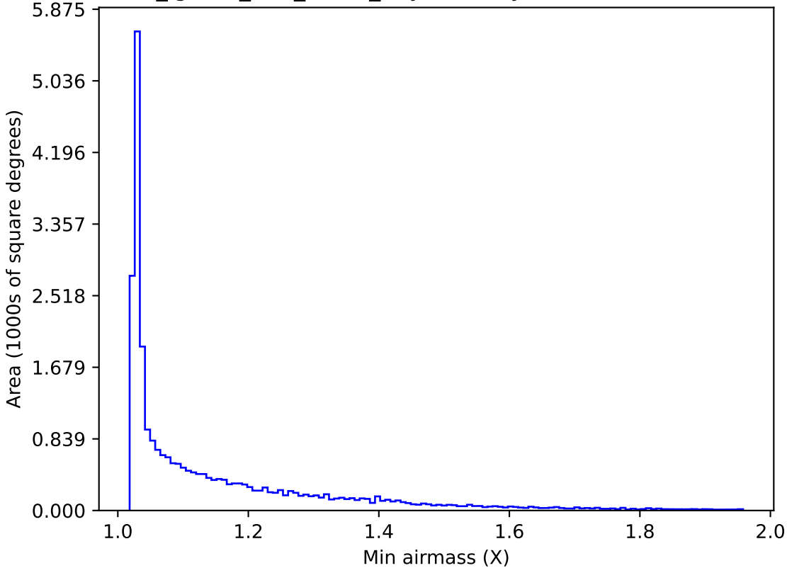
too_ignore_100_1v3.4_10yrs All sky i band: Min airmass
