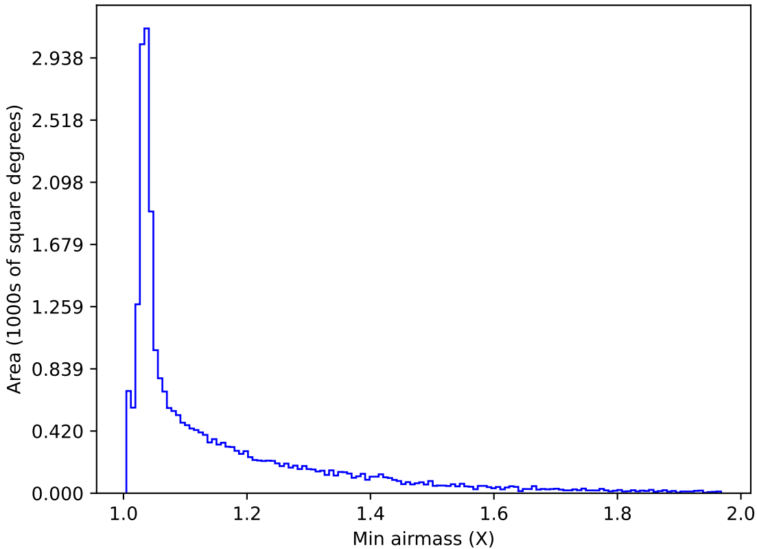
too_ignore_100_1v3.4_10yrs All sky g band: Min airmass
