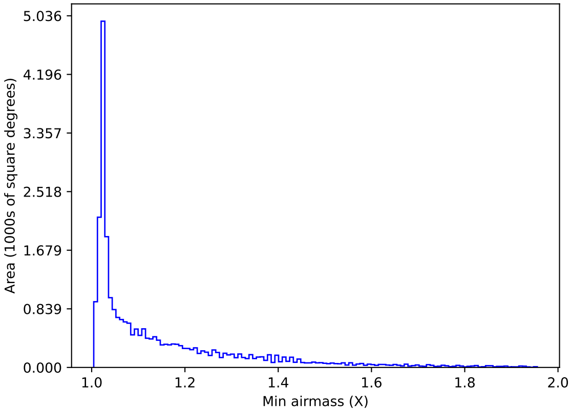
too_ignore_100_1v3.4_10yrs All sky all bands: Min airmass
