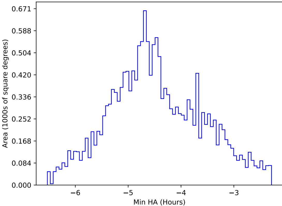
too_ignore_100_1v3.4_10yrs WFD z band: Min HA
