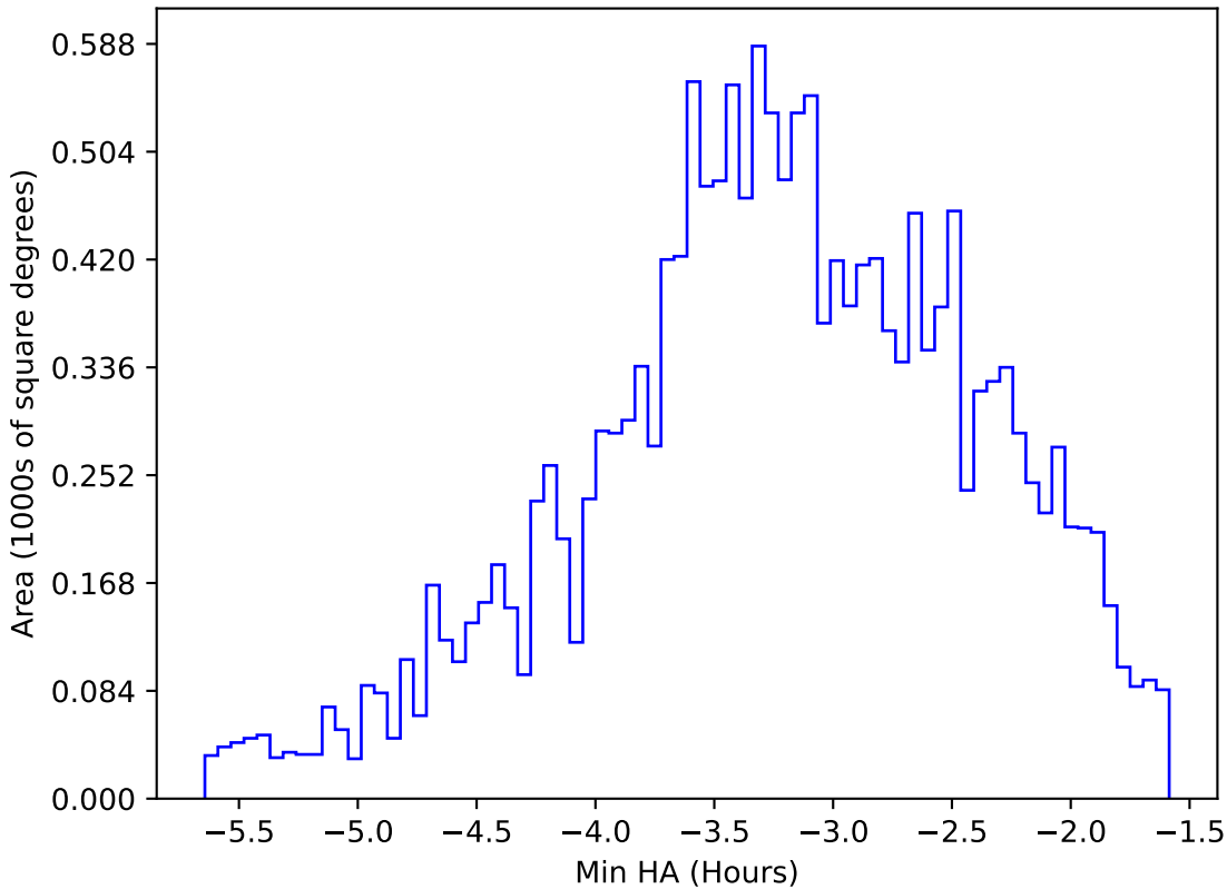
too_ignore_100_1v3.4_10yrs WFD u band: Min HA
